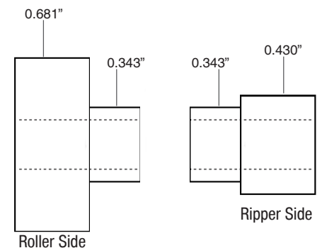
Diagram C / Bushing #PKSROLSRBU
